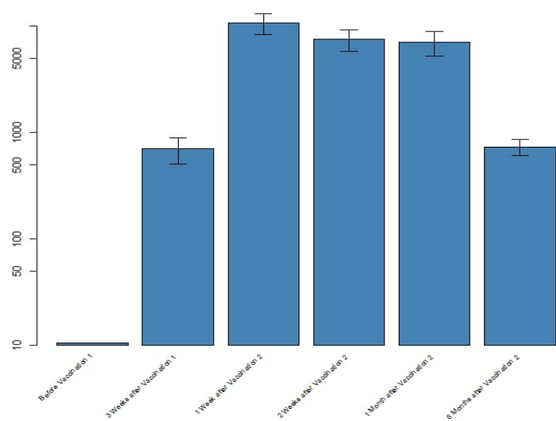
Stage 1, Age 65 - 85, BNT162b2 or placebo N= 12 (log scale)
