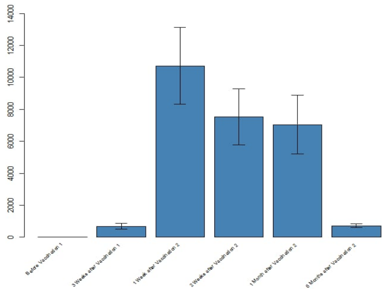
Stage 1, Age 65 - 85, BNT162b2 or placebo N= 12 (linear scale)
