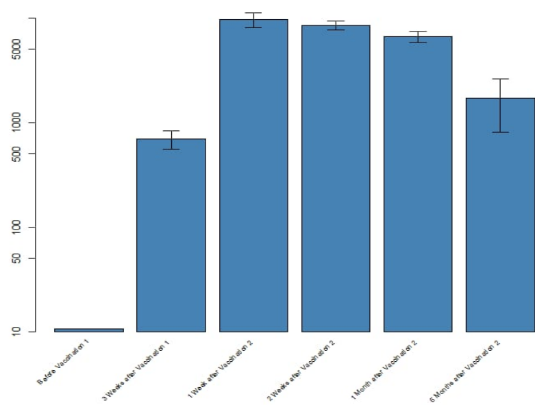
Stage 1, Age 18 - 55, BNT162b2 or placebo N= 12 (log scale)
