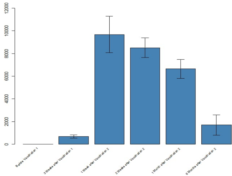
Stage 1, Age 18 - 55, BNT162b2 or placebo N= 12 (linear scale)
