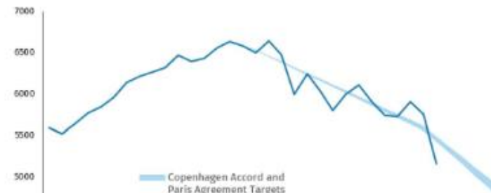
Net US GHG emissions relative to international commitments Million metric tons CO 2 e, IPCC definitions, excludes international bunkers
