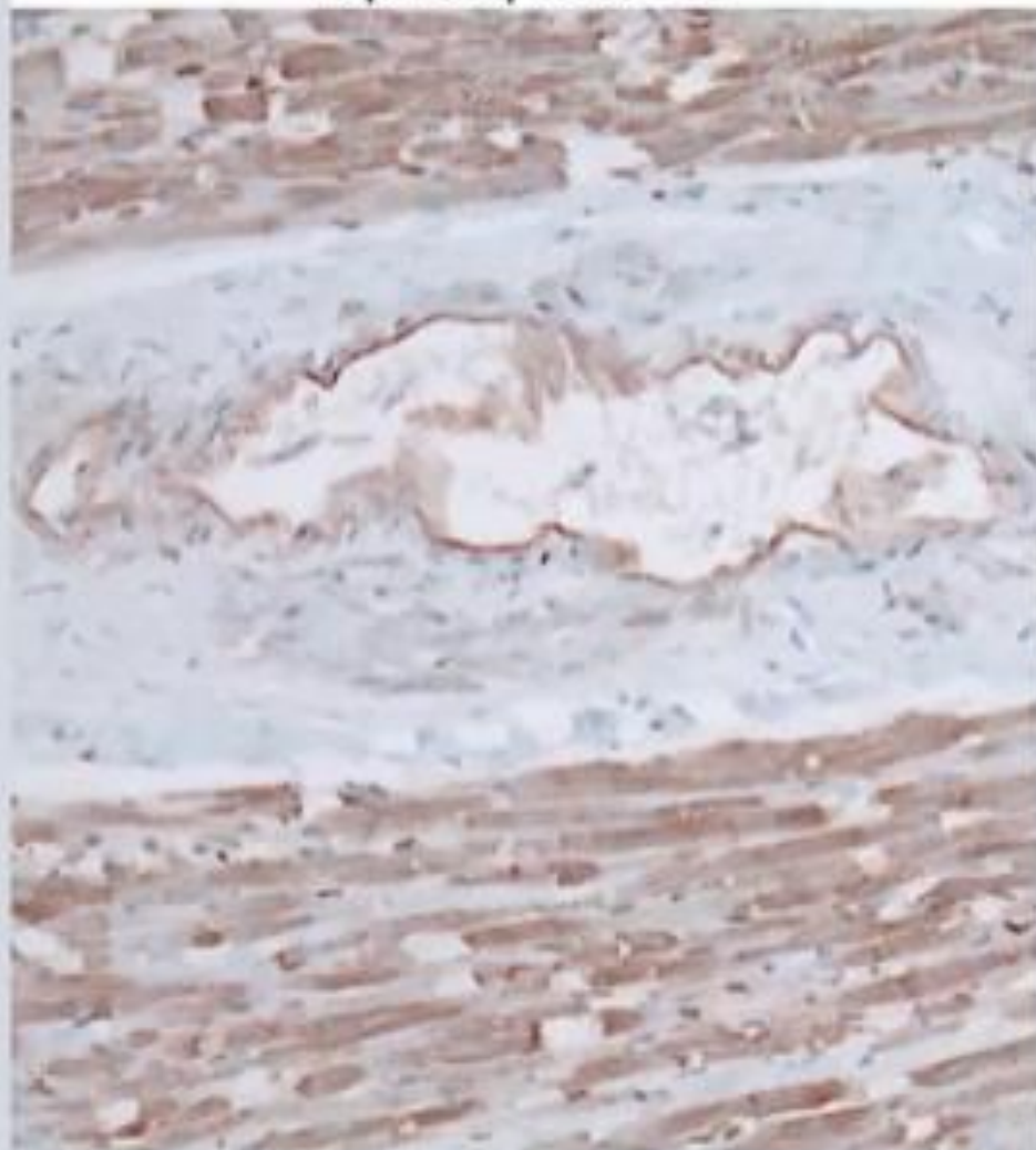
Spike protein
