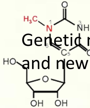
N1-methyl-Pseudouridine (N1-methyl-Ψ)
