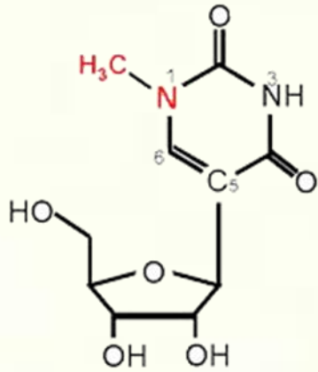
N1-methyl-Pseudouridine (N1-methyl-Ψ)
